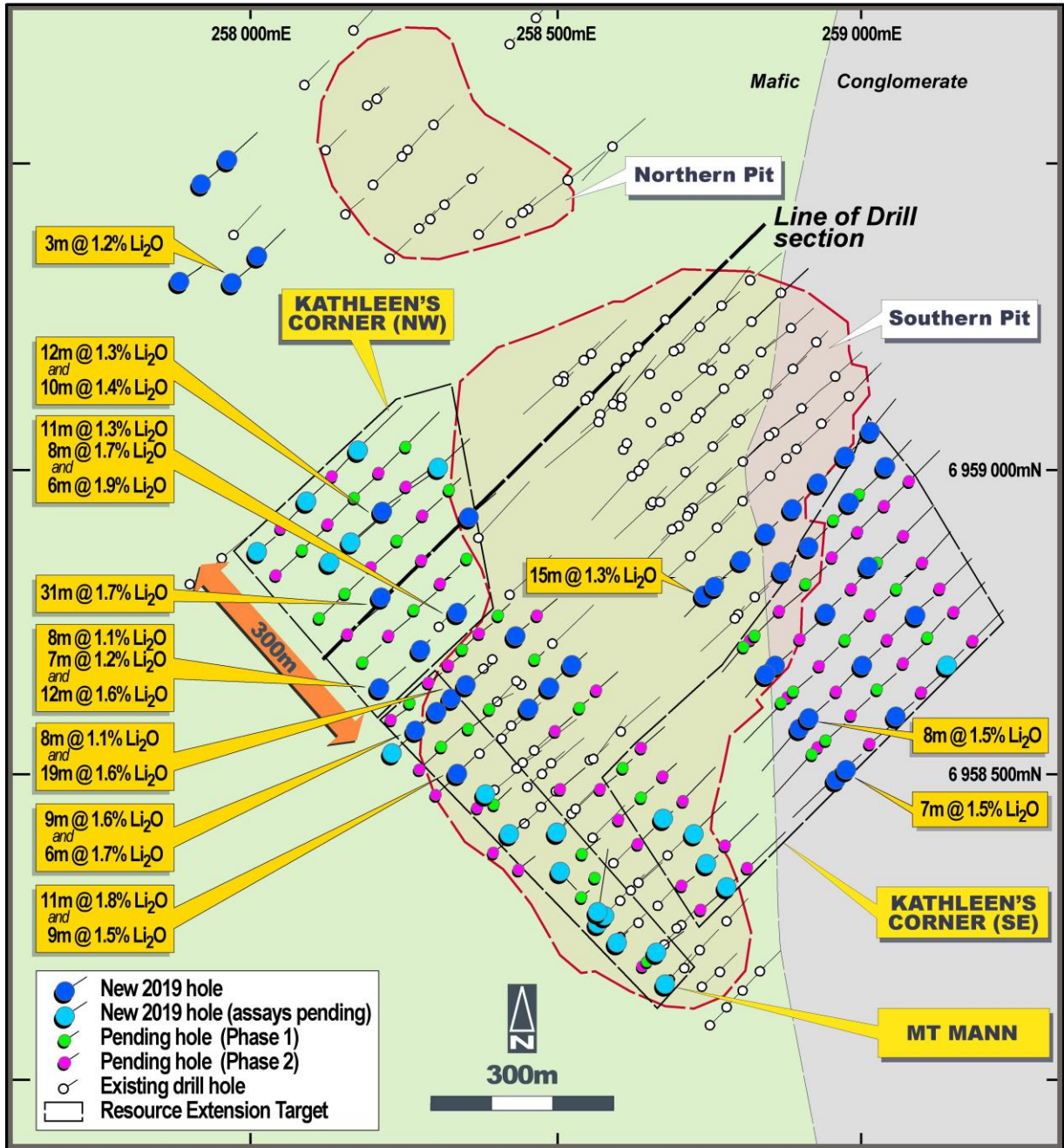
Figure 1: Kathleen Valley – Drill hole plan showing better lithium intersections from 2019 drilling program.
